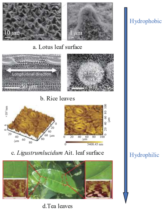
Figure 2 SEM images of the lotus leaf surface [41] and rice leaves [42] , with AFM images of Ligustrum lucidum Ait. [43] and tea leaves [16]
