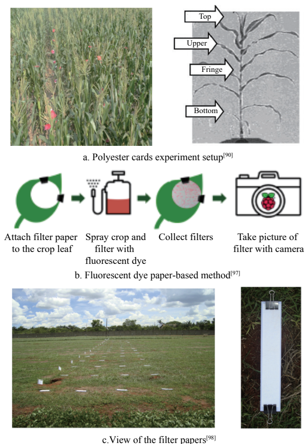
Figure 5 Measurement methods for leaf retention capacity
