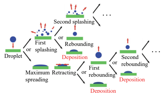
Figure 8 Schematic diagram of the impact process
