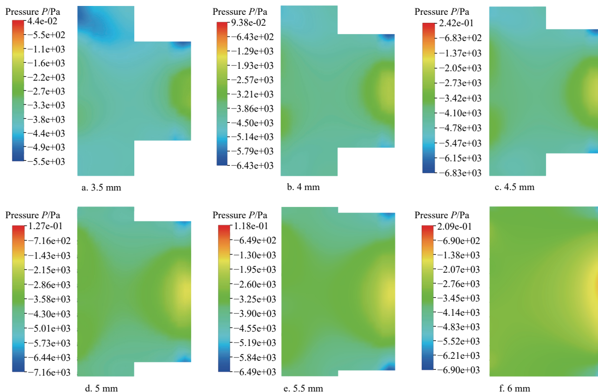
Figure 7 Pressure distributions in the suction hole
