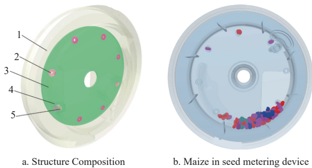
1.Front shell 2.Elastic seed suction pad 3.Seeding tray 4.Particle factory 5.Maize seed.
