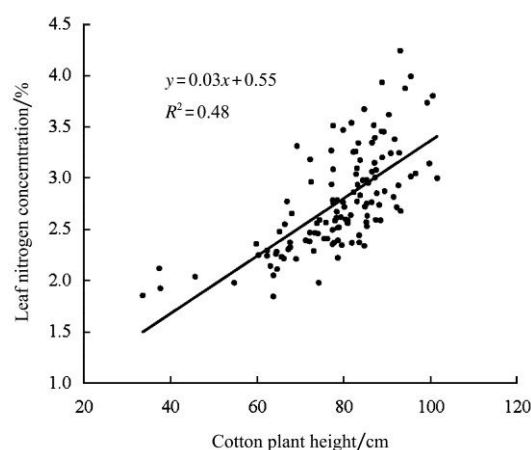
Figure 2 Relationship between leaf nitrogen content and cotton plant height determined by the ultrasonic plant height measurement system
