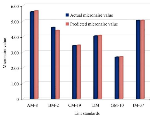
Figure 16 Actual micronaire value very strongly correlated with that predicted using the regression model involving two wavebands (1 550 nm and 1 600 nm)
