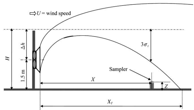
Figure 3 Illustration of the plume from a ventilation fan and the plume touching-ground distance ( X_T )
