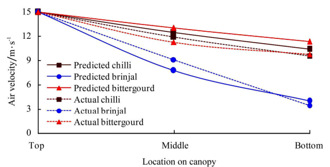
Figure 5 Comparison of air velocity in natural canopy with the predicted values
