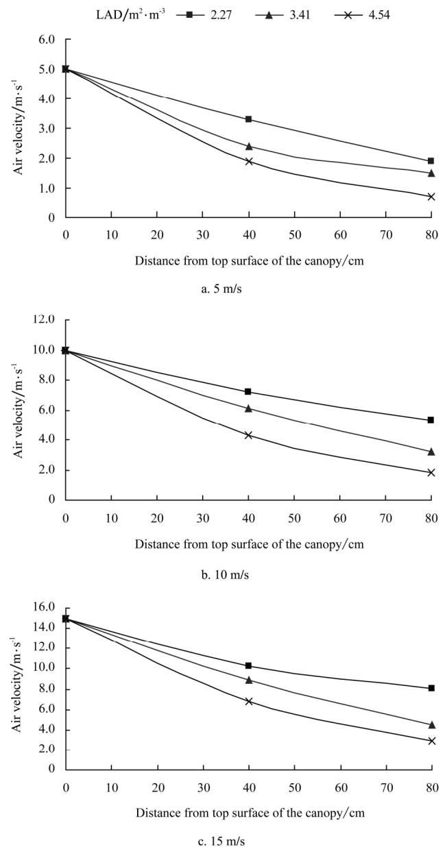
Figure 4 Effect of leaf area density (LAD) on air velocity of air stream penetrating simulated crop canopy at different speeds
