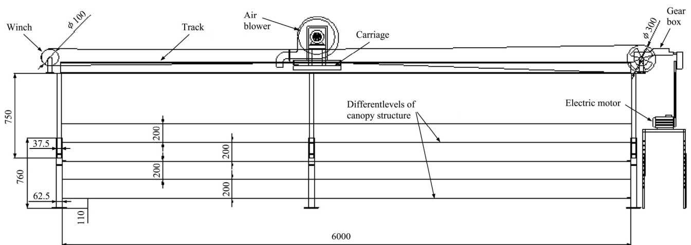
Figure 1 Schematic diagram of laboratory setup
