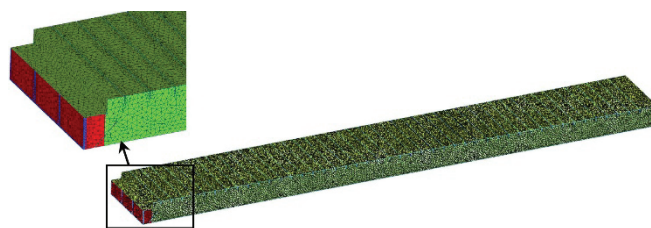
Figure 2 Model of the experimental house and surface mesh
